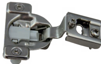
4 Way 2 Cam Adjustable 1 pc Face-Frame 105 deg Hinge w/ Dowels 1" OL H298-D H298-D-SC CASE QTY No Soft Close Soft Close 200
