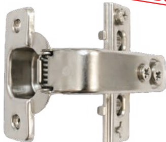
Short Arm Soft Close Inset 1pc hinge w/integrated plate 6-way CAM Adj w/ Dowel HSA3-DSC HSA3-SC CASE QTY w/ Dowels No Dowels 200
