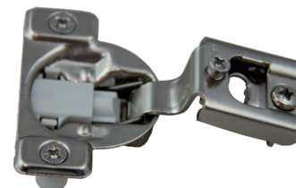
4 Way 2 Cam Adjustable 1 pc Face-Frame 105 deg Hinge w/ Dowels 1" OL H298-D H298-D-SC No Soft Close Soft Close CASE QTY 200
