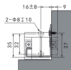
B: Plastic rear mounting bracket
