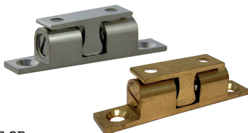
C285.SB. 2" Double Ball Catch Solid Brass CASE QTY 1,000 WEIGHT/CASE 33 lbs BOX QTY 50 Available Colors Item Number Nickel Plated C285.SB.NI Polished Brass C285.SB.PB
