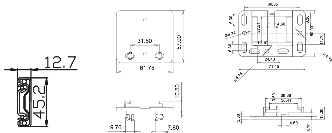
4600-BRKTPI Plug In Rear Adjustable Socket
