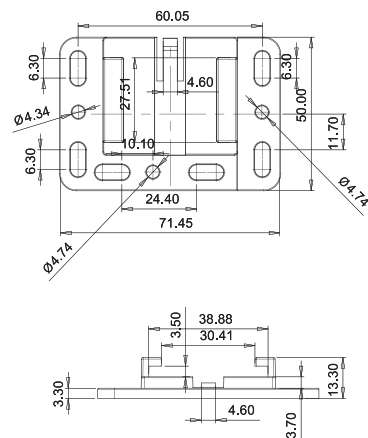
4600-BRKTSO Screw On Rear Adjustable Socket
