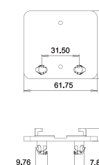
4903-BRKTPI Plug In Rear Adjustable Socket
