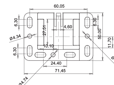
4800-BRKTPI10 Plug In Rear Adjustable Socket for 4800 Slide 10mm Dowel
