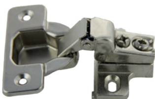
Short Arm Face Frame Hinge = 3/8" Overlay H275 No Dowels CASE QTY 200
