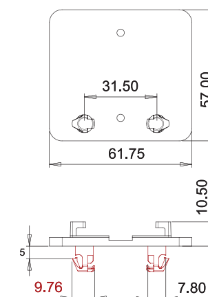
4800-BRKTPI Plug In Rear Adjustable Socket
