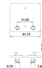
4903-BRKTPI Plug In Rear Adjustable Socket
