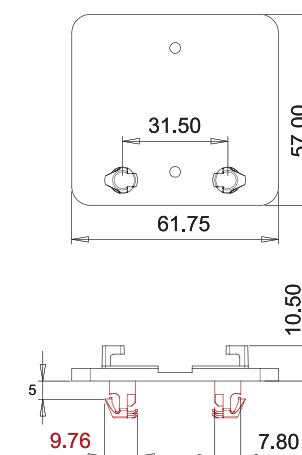
4800-BRKTPI Plug In Rear Adjustable Socket
