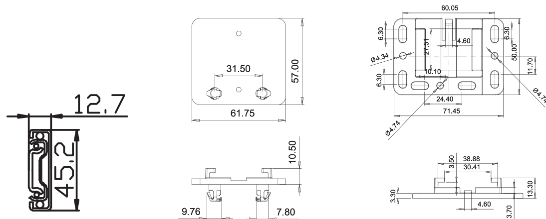
4600-BRKTPI Plug In Rear Adjustable Socket
