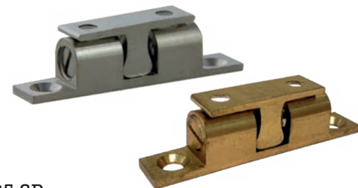
C285.SB. 2" Double Ball Catch Solid Brass CASE QTY 1,000 WEIGHT/CASE 33 lbs BOX QTY 50 Available Colors Nickel Plated Polished Brass Item Number C285.SB.NI C285.SB.PB
