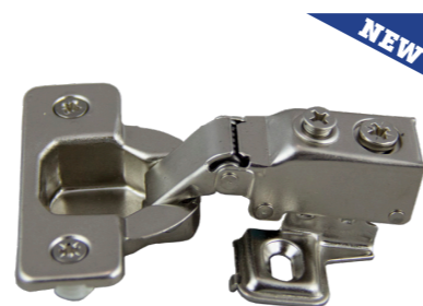
Short Arm Soft Close Face Frame CAM Hinge Steel Plate 1/2" Overlay w/ Dowel HCAM280-D-SC With Dowels
