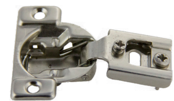
4 Way 2 Cam Adjustable 1 pc Face Frame Hinge 1/2" OL
