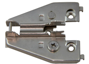
Soft Close Face Frame Plate with Cam Adjustment
